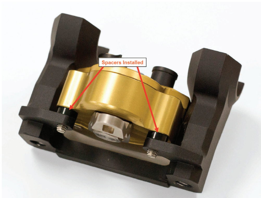
Spacers Installed
