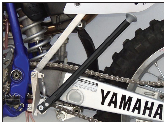
5002-YZ/WR Kickstand Installed
